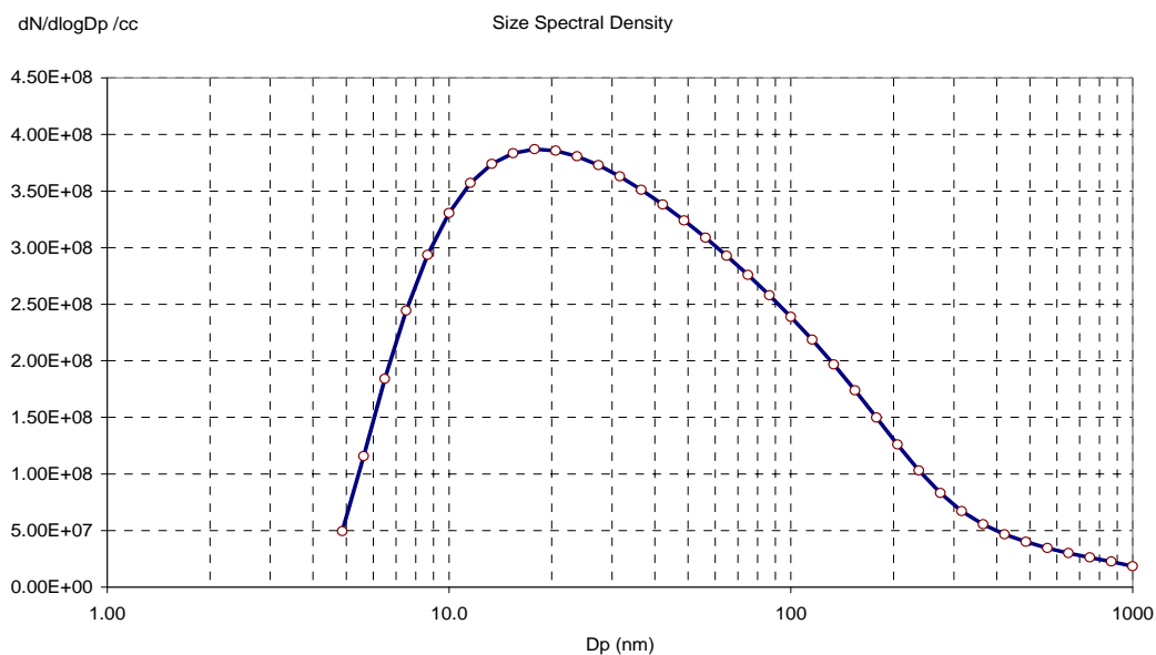
Figure 3 Spectral density of the laser toner used in experimental photocopier.
